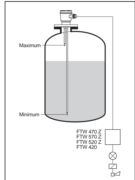
Two-point control in a metal vessel
