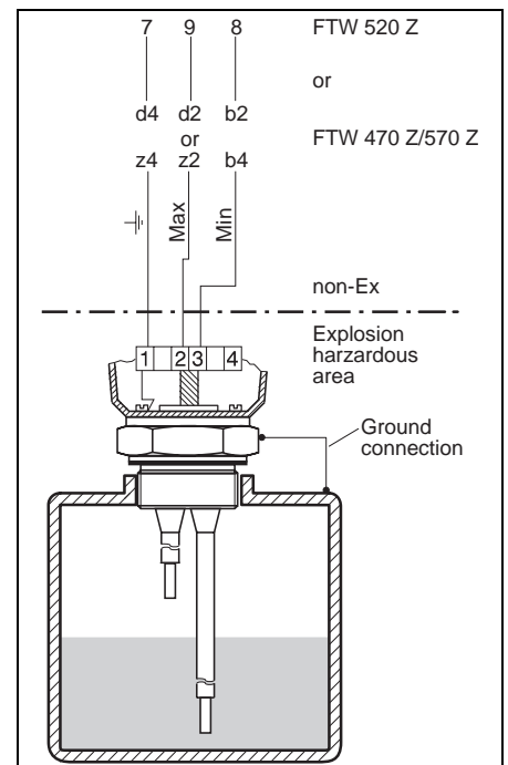
Two-point control in a metal vessel without cable monitoring and also for use in explosion hazardous areas.
