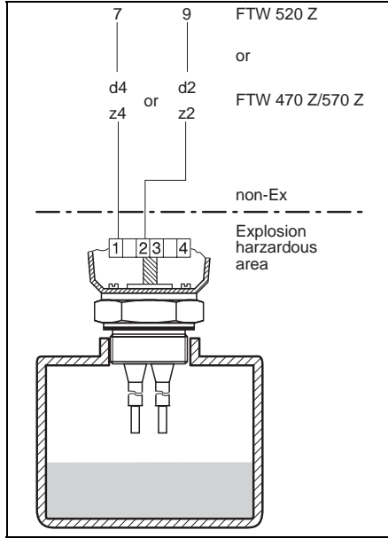
Freely selectable limit detection in a plastic vessel without cable monitoring and also for use in explosion hazardous areas.
