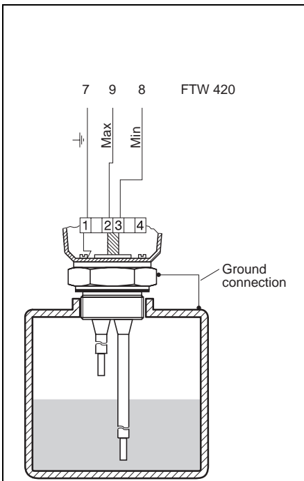
Two-point control in a metal vessel without cable monitoring.
