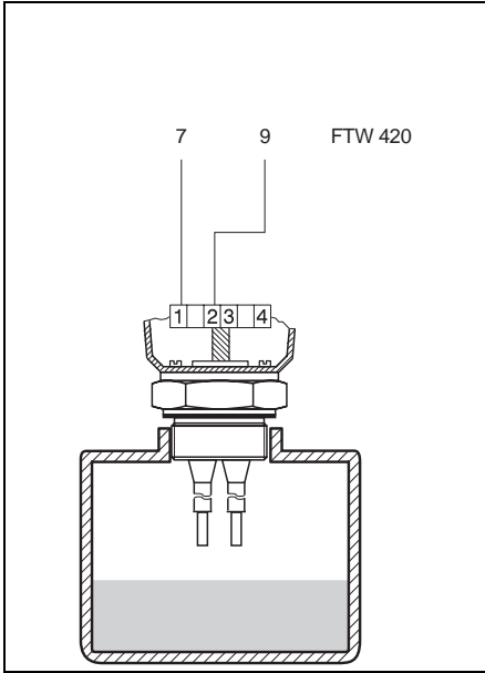
Freely selectable limit detection in a plastic vessel without cable monitoring.
