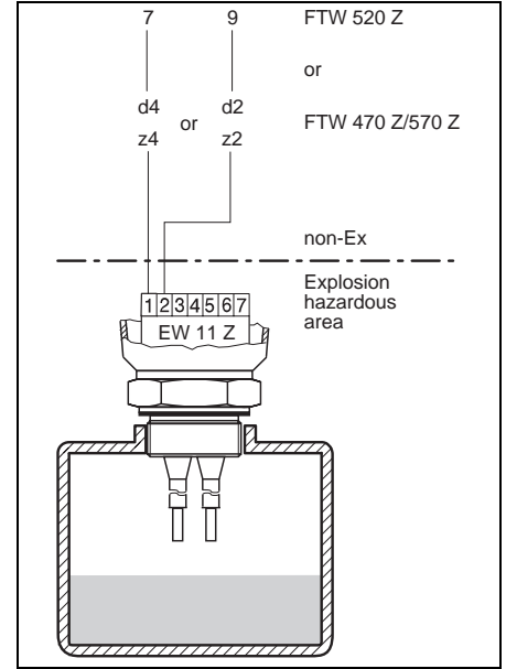
(Maximum) limit detection in a plastic vessel with cable monitoring and also for use in explosion hazardous areas.
